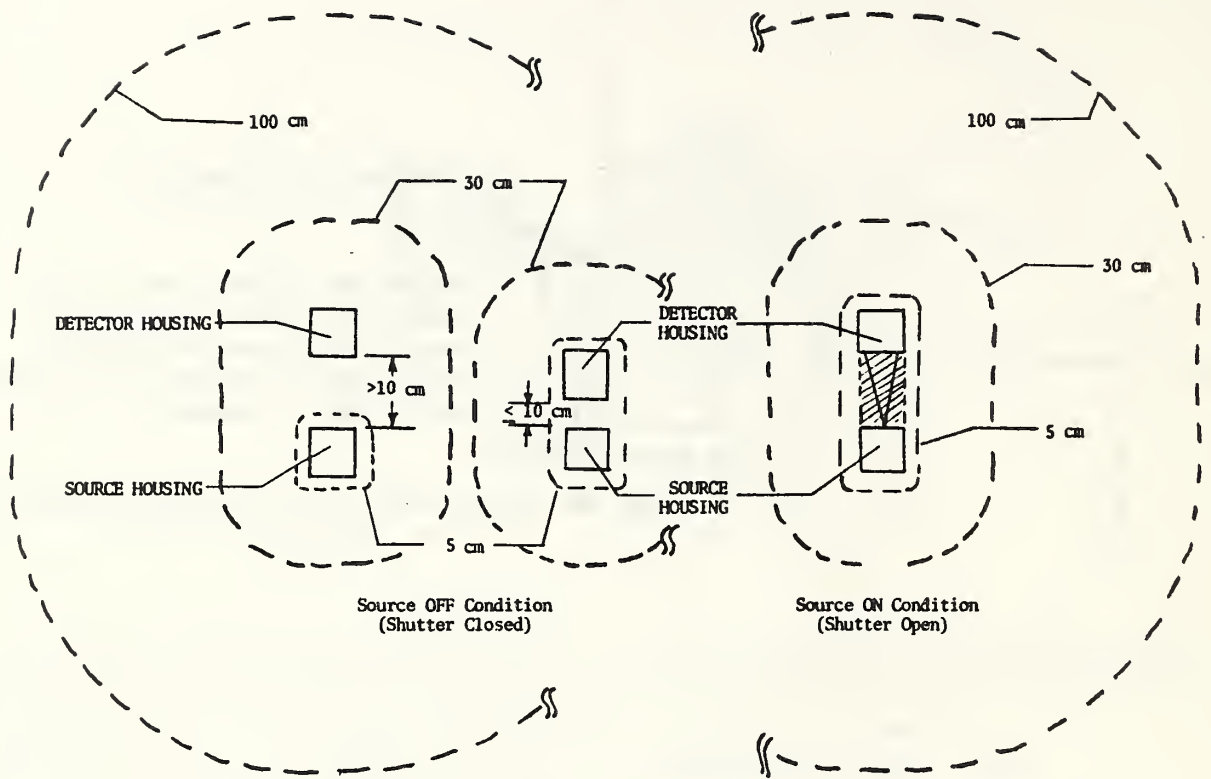
FIGURE IIC. Transmission Type Gauge (Beta, Photon, Neutron)
